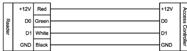
Reader mode Wiring diagram
